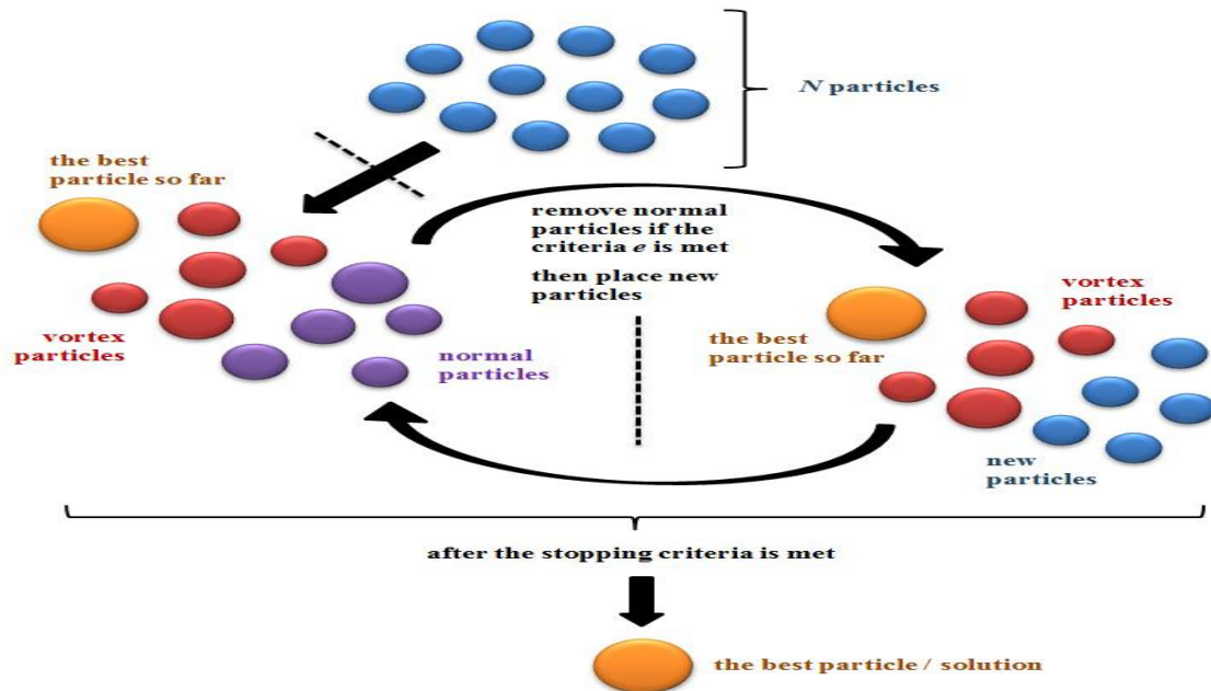
Figure 1: Operational method of the Vortex Optimization (VO) algorithm
