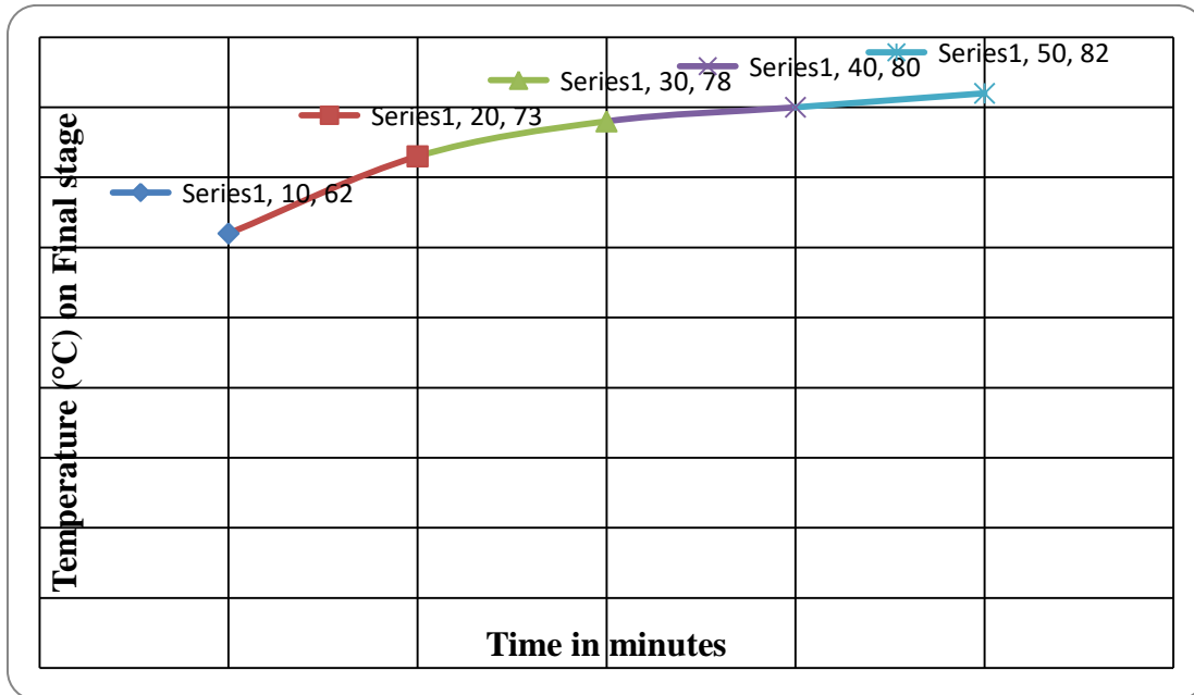
Figure 6: Testing applied load 2500 Watts
