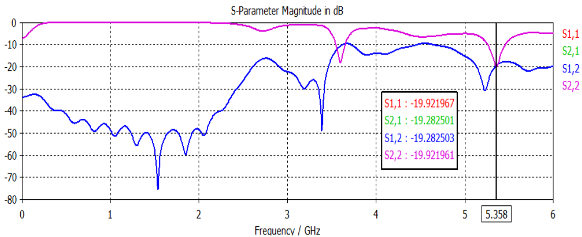
Figure 3: Simulated S-parameters of two element antenna system at 5.3 GHz
