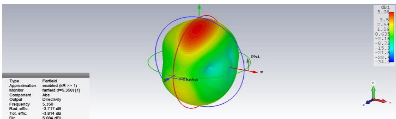
Figure 7: Directivity of MIMO antenna at 5.3 GHz
