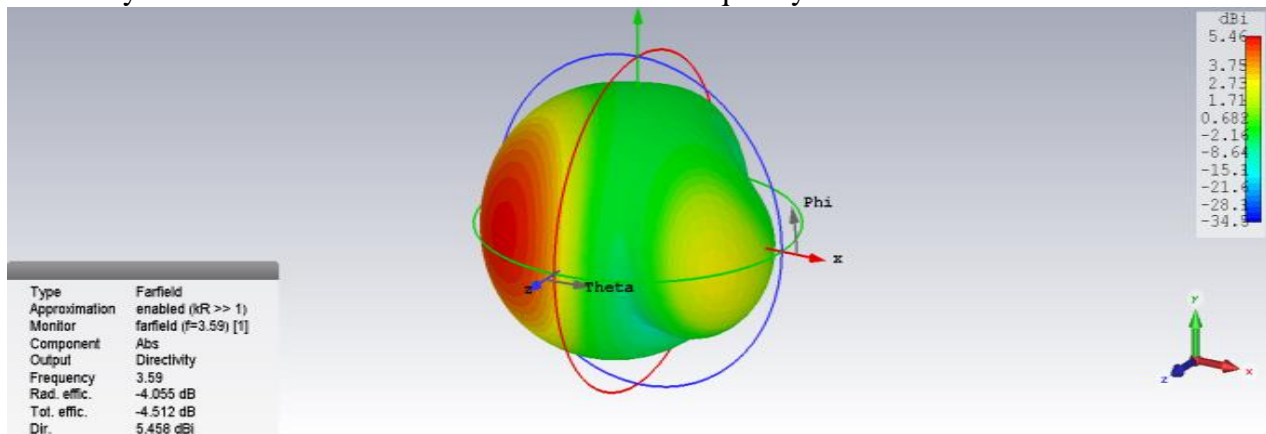
Figure 6: Directivity of MIMO antenna at 3.5 GHz
