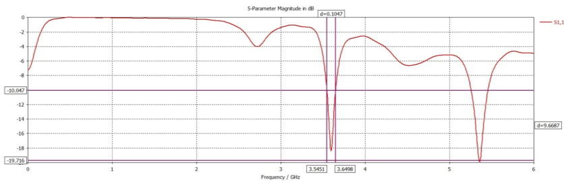
Figure 4: Bandwidth of two element antenna system at 3.5 GHz
