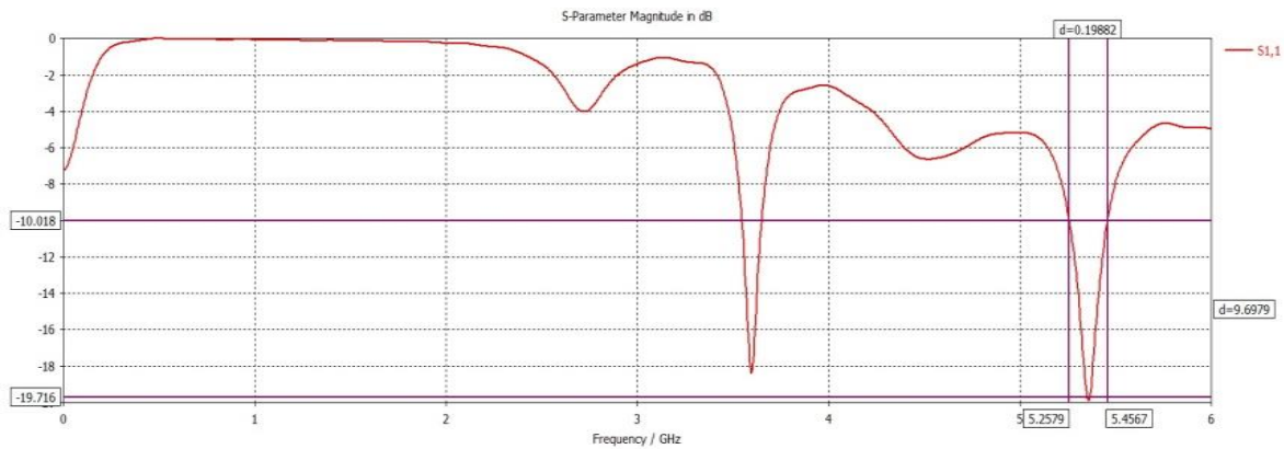
Figure 5: Bandwidth of two element antenna system at 5.3 GHz
