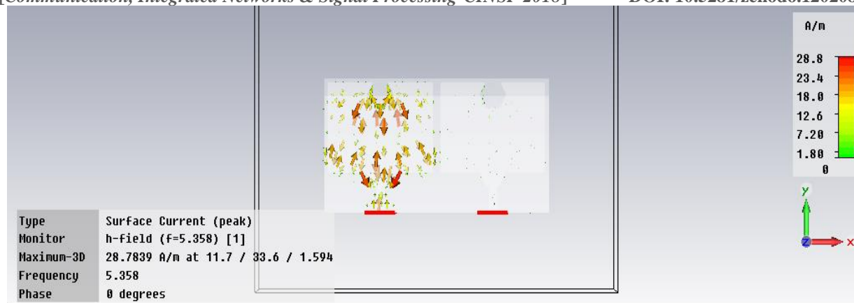
Figure 10: Surface current distributions at 5.35 GHz port 1
