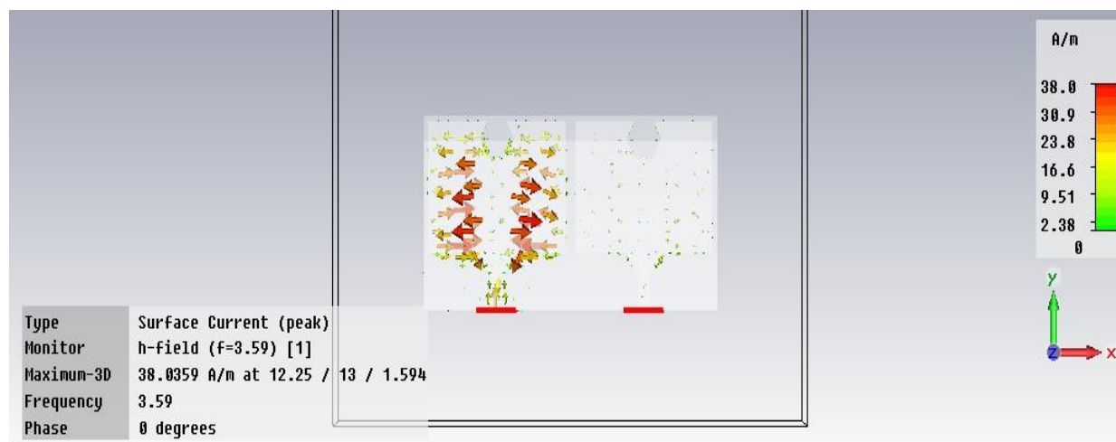
Figure 9: Surface current distributions at 3.59 GHz port 1
