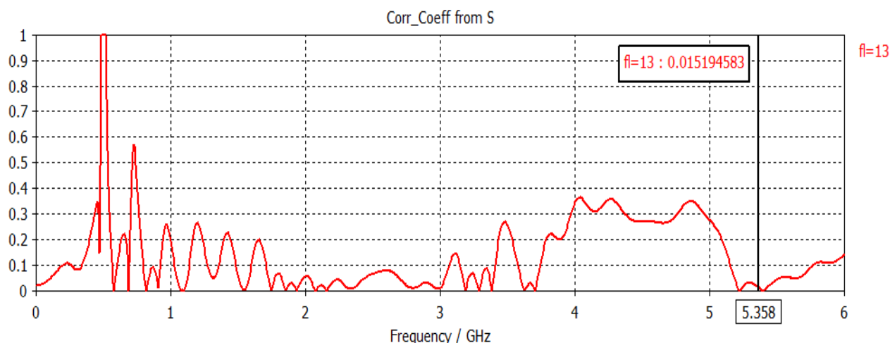
Figure 8: ECC of proposed MIMO antenna
