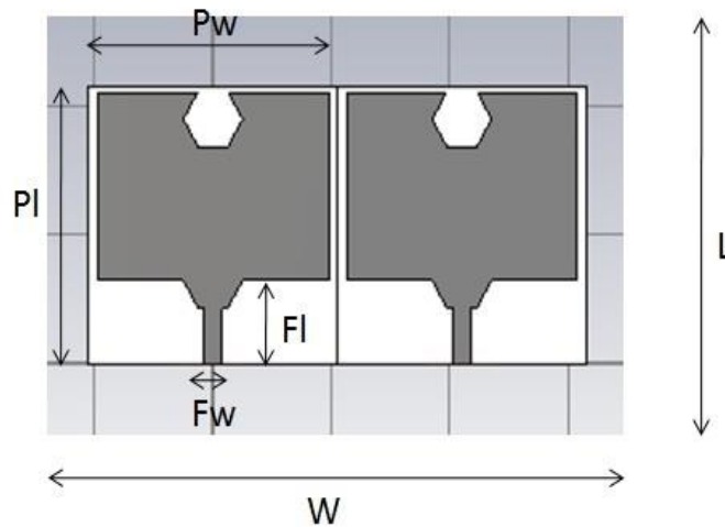
Figure 1: Proposed MIMO antenna
