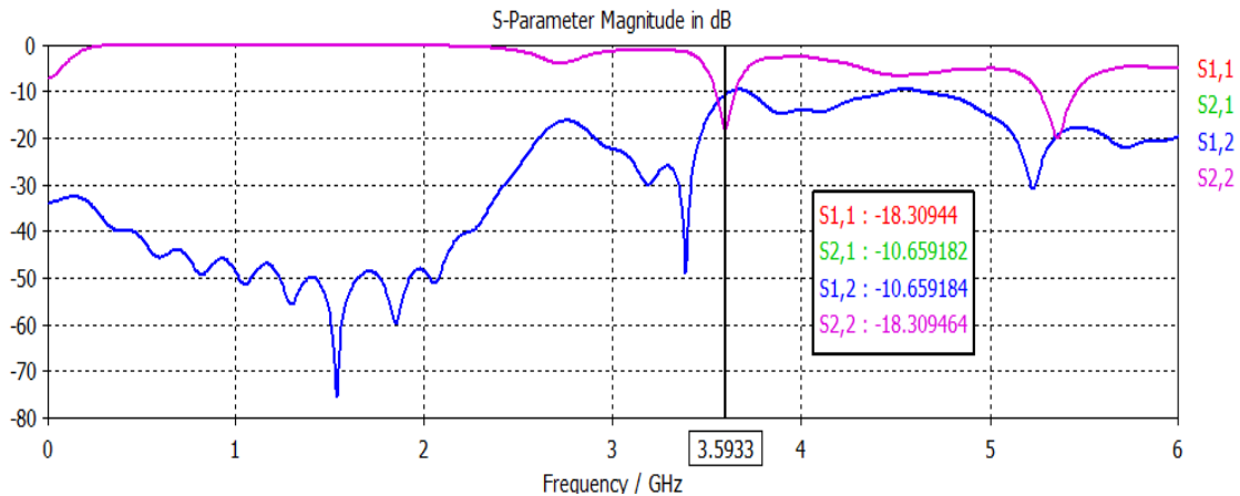
Figure 2: Simulated s-parameters of two element antenna system at 3.5 GHz.
