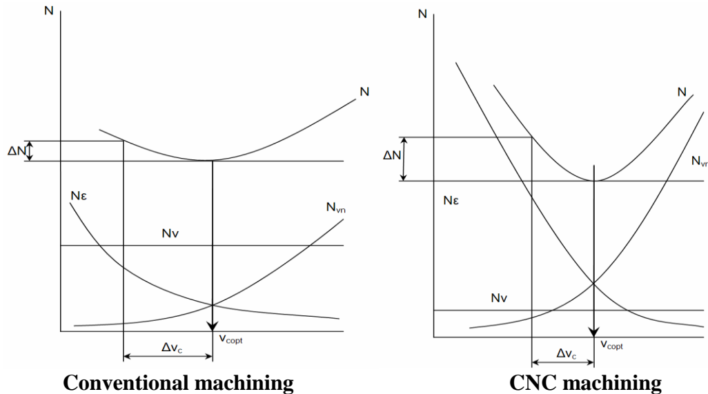
Figure 1: Dependence of N production costs and their components on cutting speed v_c . N_c – costs on machine work, N_v – secondary work costs, N_{vn} – costs to device exchange.
