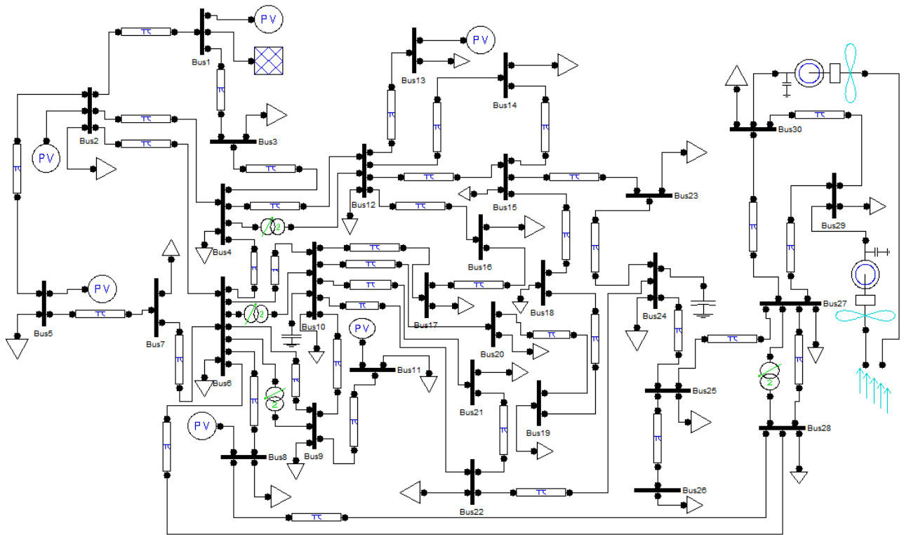
Fig.2 Load flow diagram with DG
