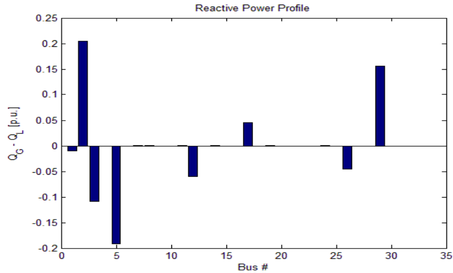
Fig.9 Reactive power profile with DG and SVC
