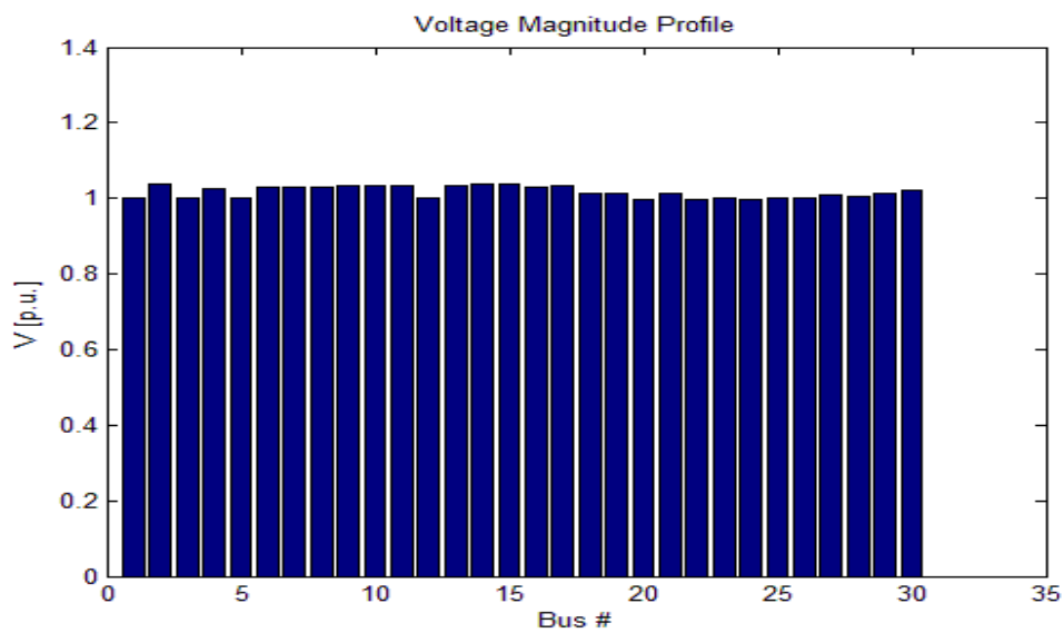
Fig.6 Voltage profile with DG and STATCOM
