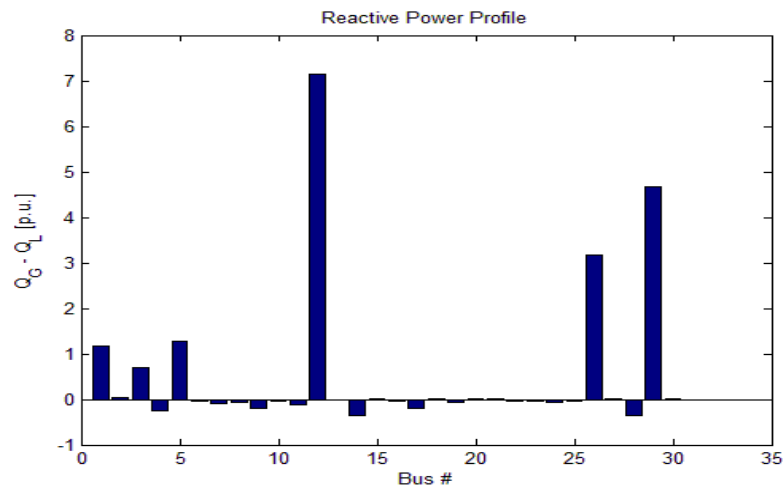
Fig.8 Reactive power profile with DG
