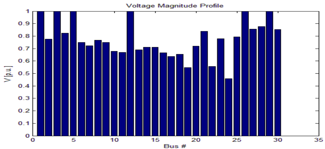
Fig.4 Voltage profile without DG connected
