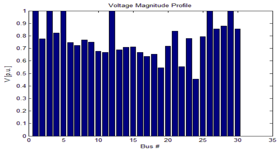
Fig.5 Voltage profile with DG connected
