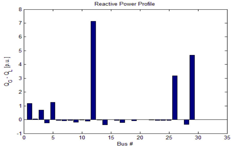
Fig.7 Reactive power profile without DG
