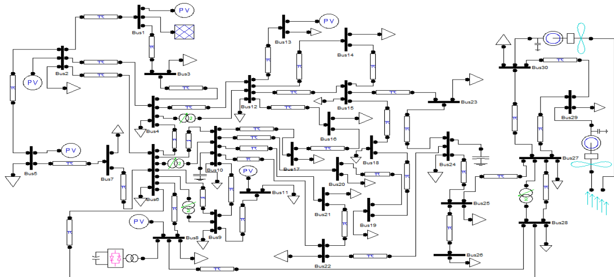
Fig.3 Load flow with DG and STATCOM
