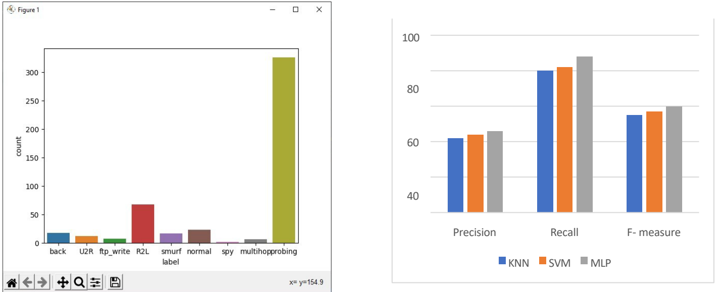
FIG 2: ATTACK TYPES
