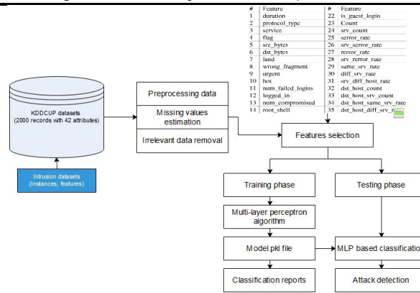
FIG 1 PROPOSED FRAMEWORK
