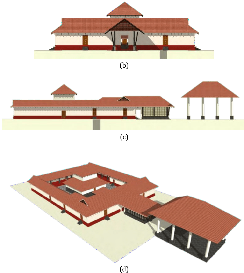
Figure 5: Thottuva Temple - (a) Dwithala Vimana - square Dravida Kerala shrine plan; (b) Front / east elevation; (c) South elevation; (d) Perspective view. Source: Authors
